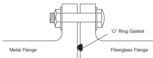
Figure 6-2 Flanged Joint
