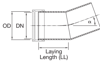
One Segmented Bend
