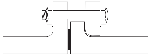
Figure 6-4 Loose Ring with Flat Gasket incl. Steel Support
