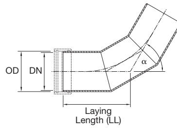
Two Segmented Bend
