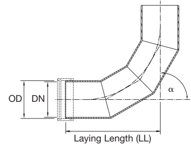
Three Segmented Bend
